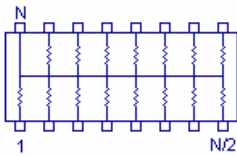
BUSSED [Schematic 1]
