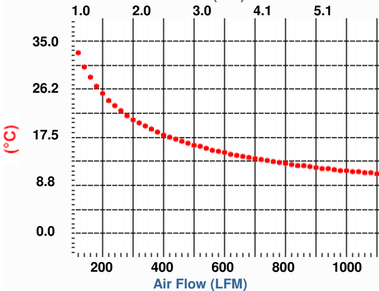
Heat Sink Temperature Rise Above Ambient (10W Dissipated)
