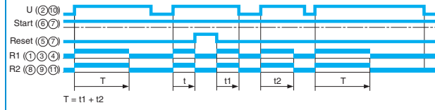
Timing on energisation, 2 timed relays
