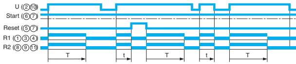
Timing on energisation, 2 timed relays
