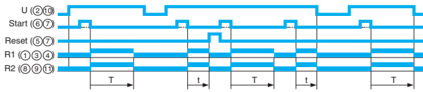
Timing after pulse on control contact, 2 timed relays
