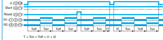
Flip-flop
