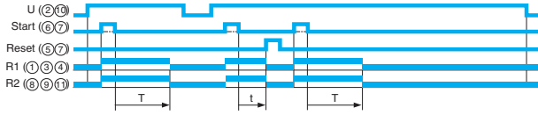
Timing after impulse (re-opening of control contact)
