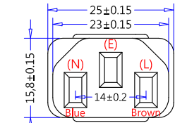
FM-5 (IEC 60320, C13, 10A 250V~) (Dimensions of Plug Face)
