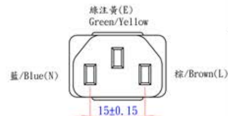
插頭端面圖 (Dimensions of Plug Face)
