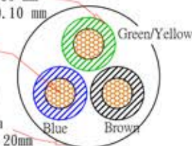
線材截面圖 (Wire Cross-Section)
