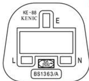
插頭端面圖 (Dimensions of Plug Face)
