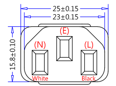
ME-302 (IEC 60320, C13, 10A 125V~) (Dimensions of Connector Face)
