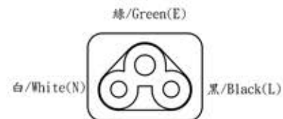
插頭端面圖 (Dimensions of Plug Face)
