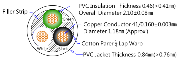
SVT 18AWGx3C截面圖 (Wire Cross-Section)
