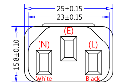
ME-302 (IEC 60320, C13) (Dimensions of Connector Face)
