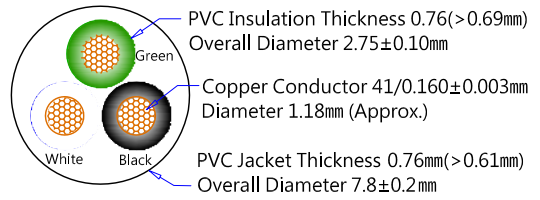
SJT 18AWGx3c 截面圖 (Wire Cross-Section)
