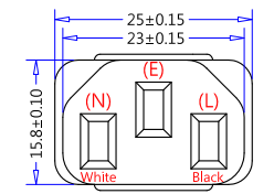
ME-302 (IEC 60320, C13) (Dimensions of Connector Face)
