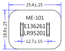
ME-101 (1-15P, Non-Polarized) (Dimensions of Plug Face)
