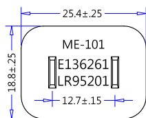
ME-101 (1-15P, Non-Polarized) (Dimensions of Plug Face)
