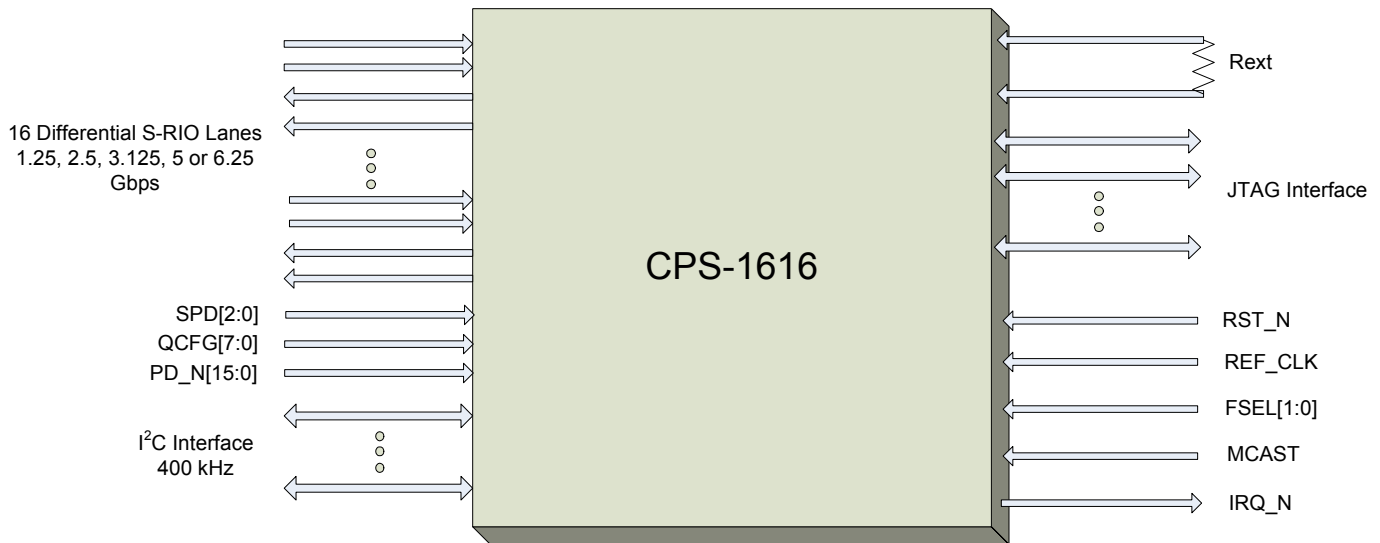
Figure 2: CPS-1616 Interfaces
