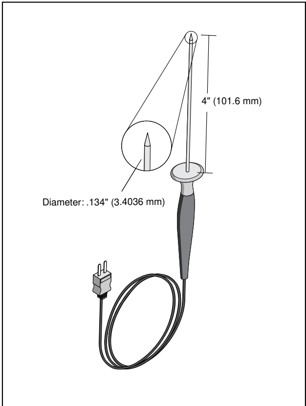
Figure 1. 80PT-25
