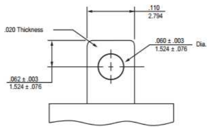
Enlarged View B
