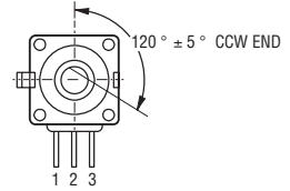
FLATTED SHAFT
