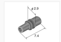
0.64mm 7165-1199
