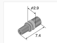
0.64mm 7165-1198
