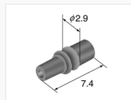
0.64mm 7165-1312
