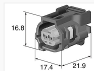
0.64mm 6189-7020
