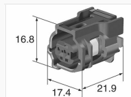
0.64mm 6189-1161
