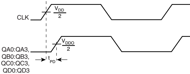
PROPAGATION DELAY
