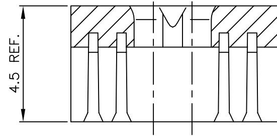
SECTION Z-Z
