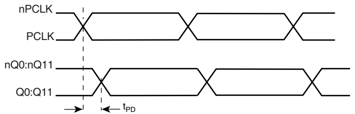
PROPAGATION DELAY
