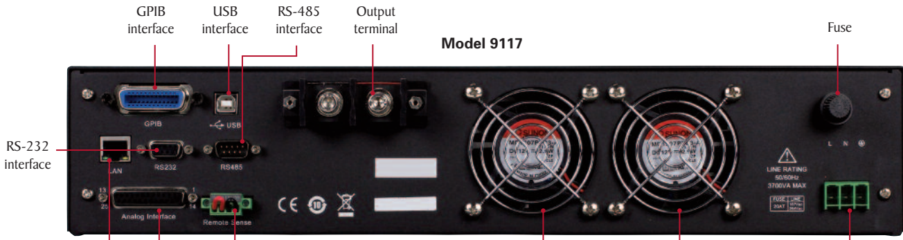
Remote sense terminal Output terminal Cooling fan USB interface RS-485 interface Cooling fan Fuse Analog control interface GPIB interface RS-232 interface AC line input
