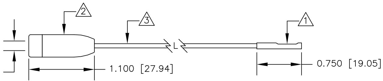
∅0.163 [4.13] X 0.625 [15.88] DP. BANANA SOCKET
