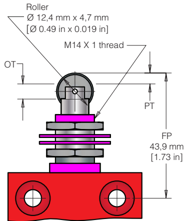
Figure 9. 924CE28 Dimensions
