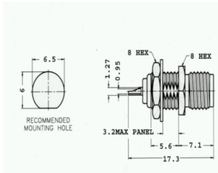
PC Board / Panel Mount Types Bulkhead Jack Front Mount P/N: 926A515
