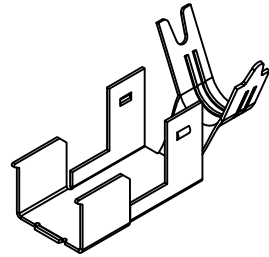
REAR SHELL
