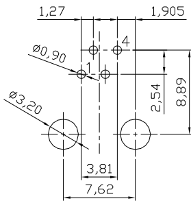
PC Board Layout Component Side Shown
