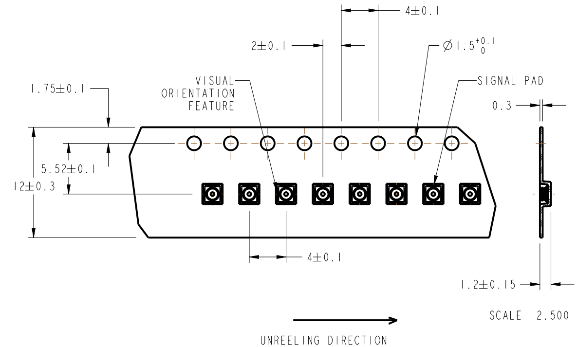
EMBOSSD CARRIER TAPE DIMENSIONS
