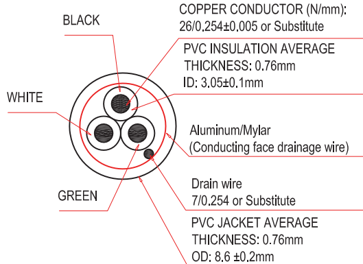
Wire cross section
