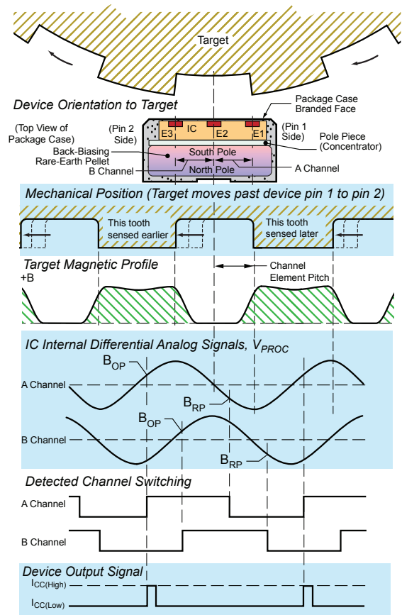
Figure 4: The magnetic profile reflects the features of the target, allowing the sensor IC to present an accurate digital output (-xSxxx variant shown).
