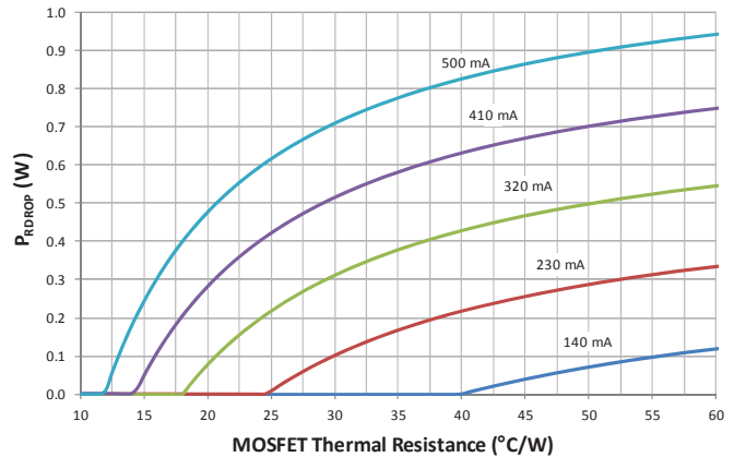
Figure 9. R_{DROP} Dissipation versus MOSFET thermal resistance at various V33 regulator maximum current settings, I_{V33ILIM}
