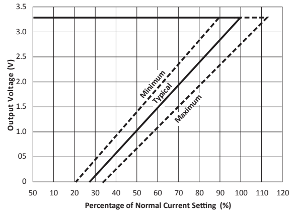
Figure 7. Foldback current limit of the V33 regulator
