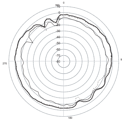
..... vertical pol phi 90 ——— horiz pol phi 90 ——— total field phi 90
