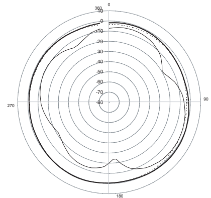
..... horiz pol theta 90 ——— vert pol theta 90 ——— total field theta 90
