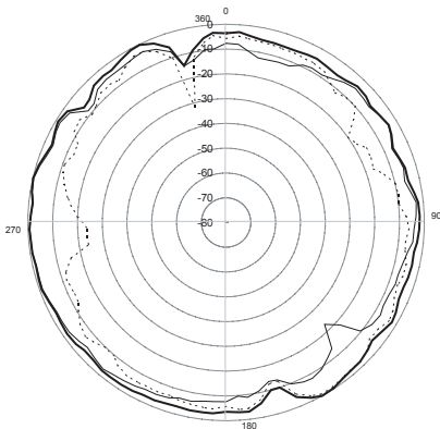
..... horiz pol phi 0 ——— vert pol phi 0 ——— total field phi 0
