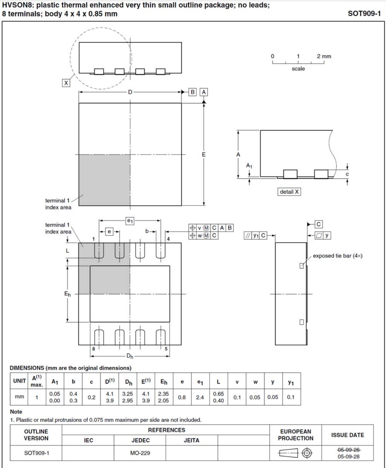
Fig 5. Package outline SOT909-1
