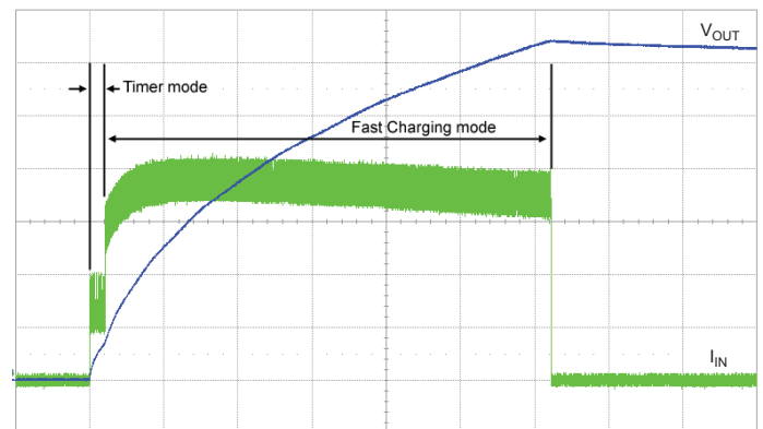
Figure 2. Timer mode and Fast Charging mode: t = 1 s/div; V_{OUT} = 50 V/div; I_{IN} = 100 mA/div., V_{IN} = V_{BAT} = 3.6 V; C_{OUT} = 100 \mu F /330 V; and I_{LIM} = 1.0 A.
