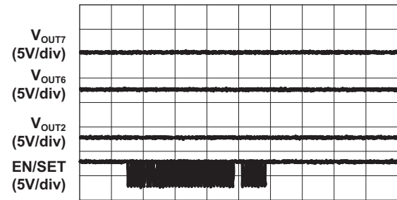
Time (10µs/div)
