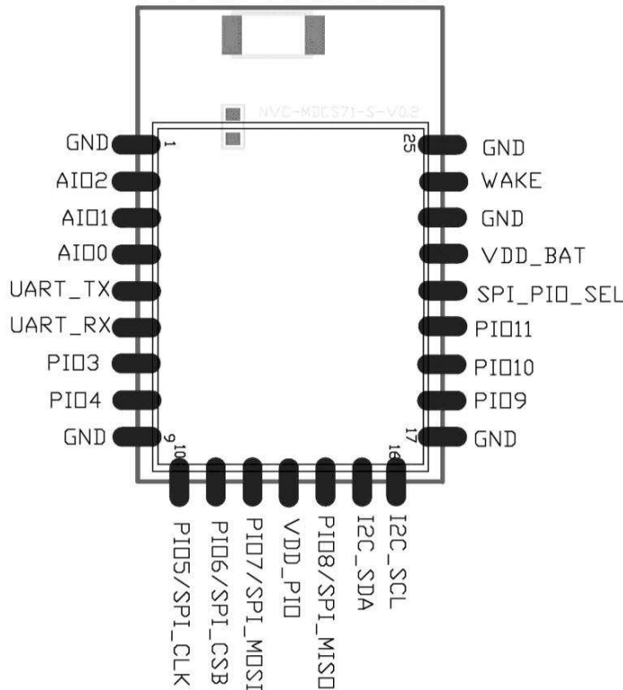
Figure 1. Pinout (Topview)
