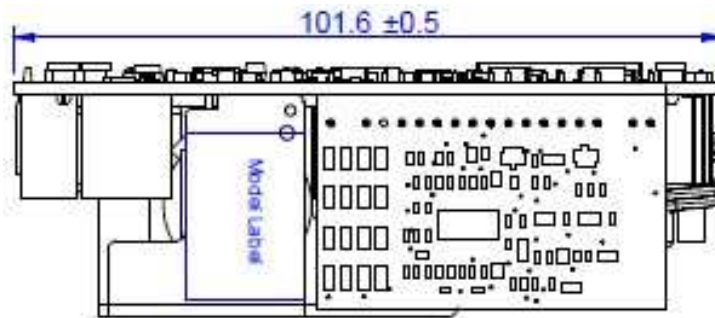
Figure 16. Side view 2
