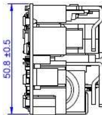
Figure 18. Front view
