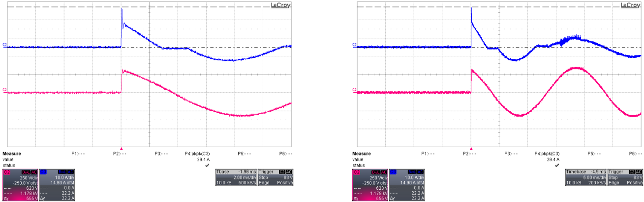
Figure 3: Inrush current, V_{in} = 230V_{ac} , 90° CH2: V_{in} (250V/div), CH3: i_{in} (10A/div)
