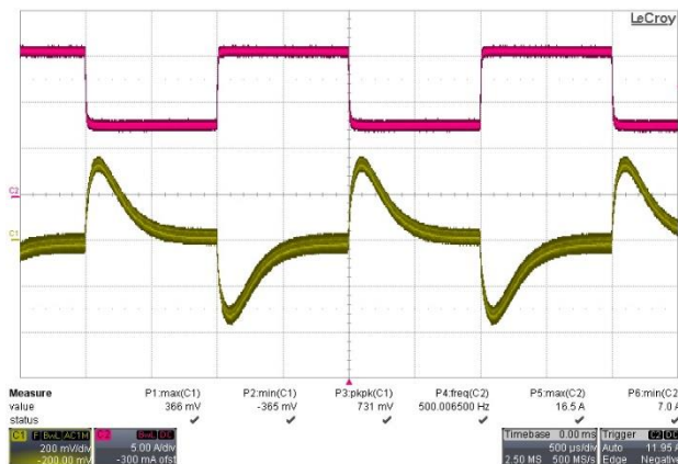
Figure 13: Load transient V_o (500µs/div), 8.5A <-> 17A 2A/µs
