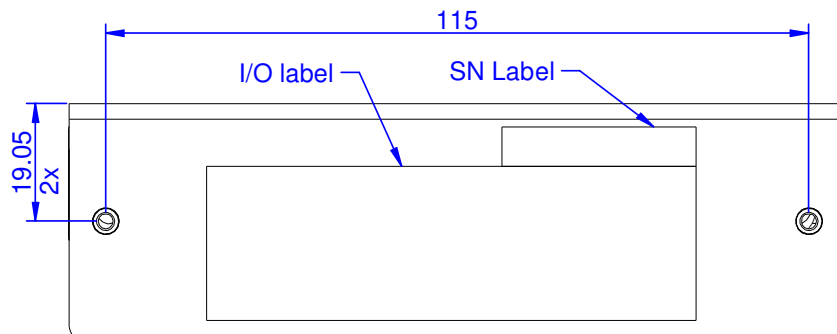
Figure 18: Side view 2
