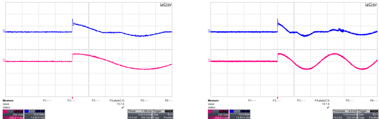
Figure 2: Inrush current, V_{in} = 115\text{Vac} , 90^\circ\text{CH2} : V_{in} (250V/div), \text{CH3} : I_{in} (10A/div)
