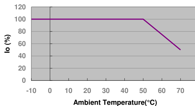
Figure 15: Output Current Limitation Curve
