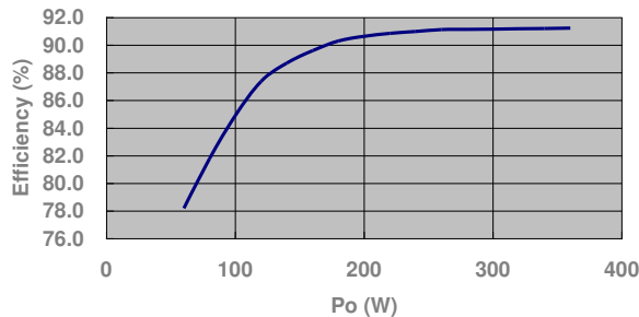
Figure 4: Efficiency vs. Output Power at 230VAC, ABC400-1012G
