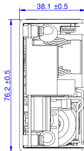
Figure 21: Front view
