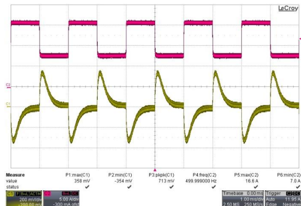
Figure 14: Load transient V_o (1.0ms/div), 8.5A <-> 17A, 2A/µs
