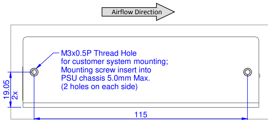
Figure 17: Side view 1
