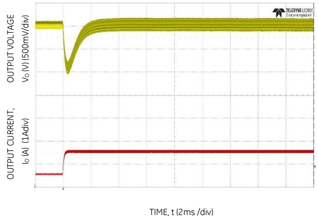
Figure 10. Transient Response to Dynamic Load Change from 0.6 to 1.6A at 12Vin, Cout=10x4.7uF, CTune=560pF, RTune=40.2k
