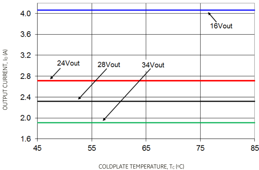
Figure 34. Output Current versus Coldwall Temperature; V_{IN} = 12V .
