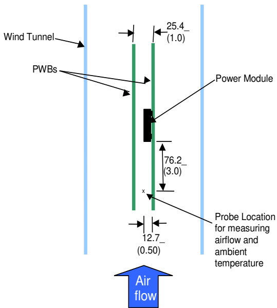
Figure 32. Thermal Test Setup.
