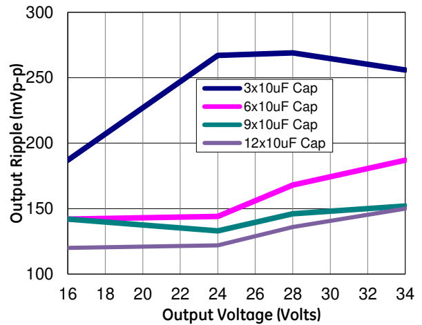
Figure 26. Output ripple voltage .Input voltage is 12V. Scope BW Limited to 20MHz
