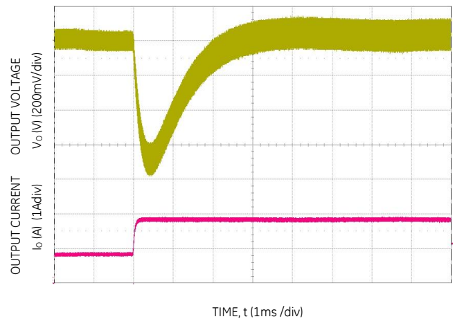
Figure 22. Transient Response to Dynamic Load Change from 0.9A to 1.9A at 12V in , C out =9x10uF, C Tune =1000pF, R Tune =30.1kΩ
