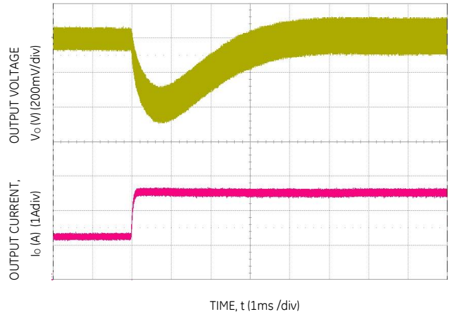
Figure 10. Transient Response to Dynamic Load Change from 50% to 100% at 12Vin, C out =3x10uF+220uF, C Tune =3300pF, R Tune =30.1kΩ
