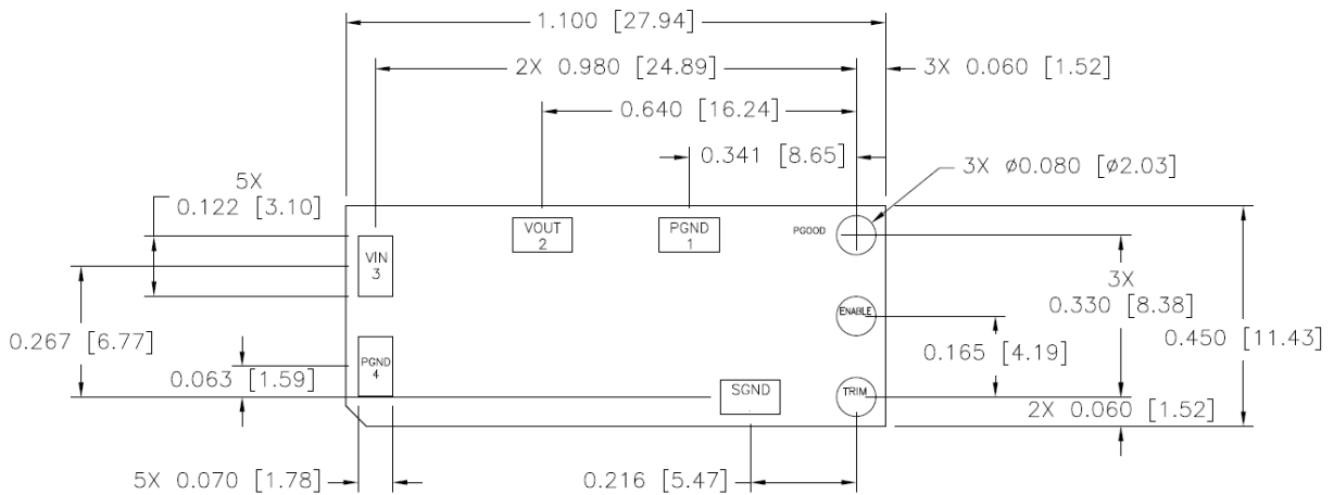
MODULE'S PWB FOOTPRINT LAYOUT (BOTTOM VIEW)
