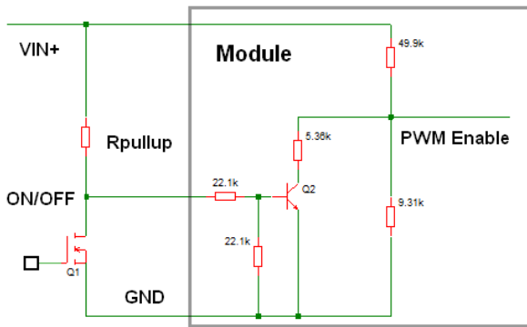
Figure 27. Circuit configuration for using negative On/Off logic.
