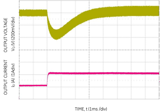
Figure 16. Transient Response to Dynamic Load Change from 50% to 100% at 12Vin, Cout=9x10uF, CTune=3300pF, RTune=30.1kΩ
