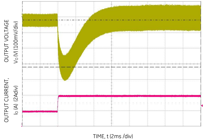
Figure 4. Transient Response to Dynamic Load Change from 50% to 100% at 12Vin, C out =3x10uF+220uF, C Tune =6800pF, R Tune =30.1kΩ
