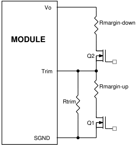
Figure 30. Circuit Configuration for margining Output voltage.
