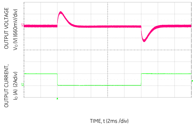
Figure 4. Transient Response to Dynamic Load Change from 50% to 0% at 12Vin, C out =3x10uF+470uF, C Tune =1000pF, R Tune =30.1kΩ
