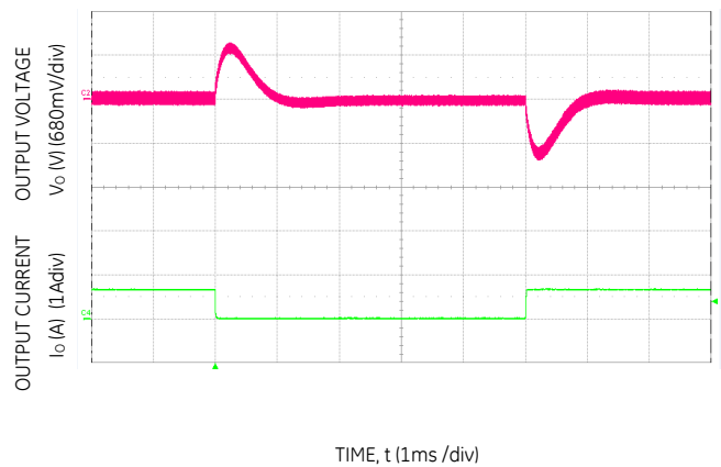
Figure 16. Transient Response to Dynamic Load Change from 50% to 0% at 12Vin, Cout=470uF, CTune=1000pF, RTune=30.1kΩ
