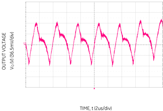
Figure 3. Typical output ripple and noise (C o =3x10uF+470uF, V IN = 12V, I o = I o,max .)
