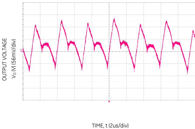
Figure 15. Typical output ripple and noise(C o =3x10uF+470uF, VIN = 12V, I o = I o,max ).
