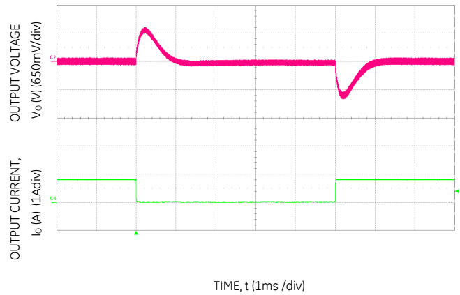
Figure 10. Transient Response to Dynamic Load Change from 50% to 0% at 12Vin, Cout=3x10uF+470uF, CTune=1000pF, RTune=30.1kΩ
