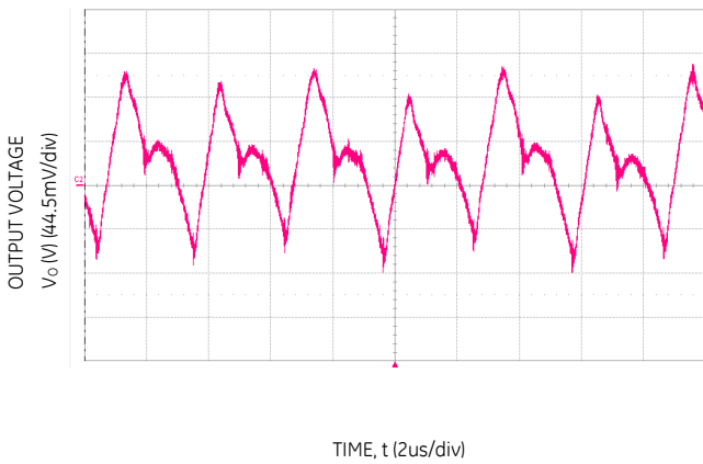
Figure 9. Typical output ripple and noise (Co=3x10uF+470uF, VIN = 12V, Io = Io,max.).
