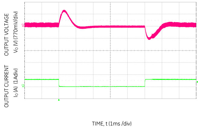
Figure 22. Transient Response to Dynamic Load Change from 50% to 0% at 12Vin, C out =470uF, C Tune =1000pF, R Tune =30.1kΩ
