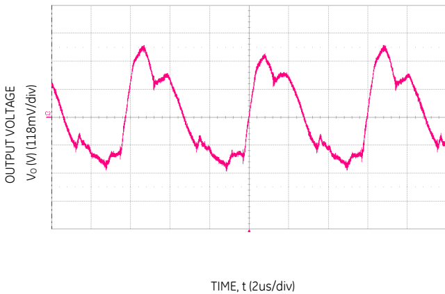
Figure 21. Typical output ripple and noise (C o =3x10uF+470uF, V IN = 12V, I o = I o,max ).
