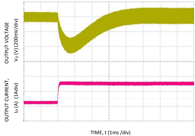
Figure 10. Transient Response to Dynamic Load Change from 50% to 100% at 12Vin, C_{out}=3 \times 10 \mu\text{F} + 470 \mu\text{F} , C_{Tune}=1000 \text{pF} , R_{Tune}=30.1 \text{k}\Omega
