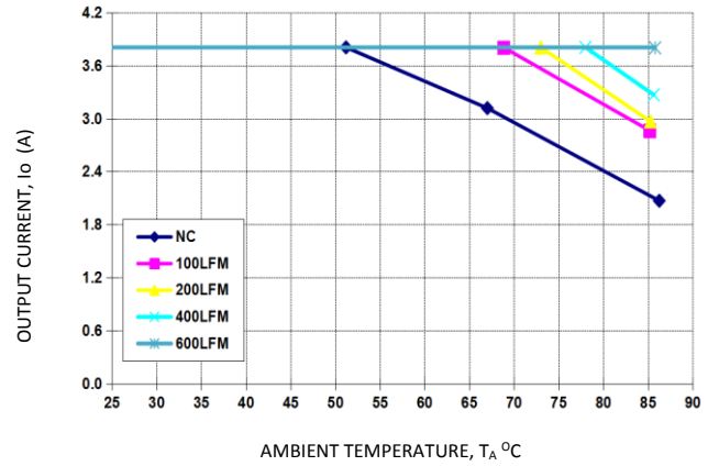
Figure 20. Derating Output Current versus Ambient Temperature and Airflow. VIN = 12V
