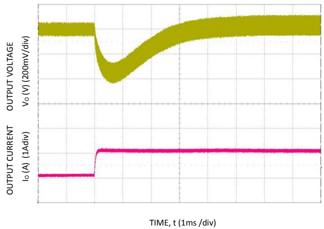
Figure 16. Transient Response to Dynamic Load Change from 50% to 100% at 12Vin, C_{out}=470 \mu\text{F} , C_{Tune}=1000 \text{pF} , R_{Tune}=30.1 \text{k}\Omega
