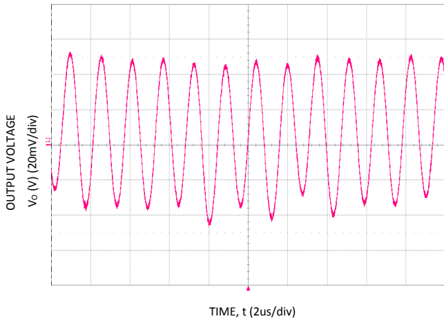
Figure 3. Typical output ripple and noise ( C_o=3 \times 10\mu F + 470\mu F , V_{IN} = 12V , I_o = I_{o,max} ).
