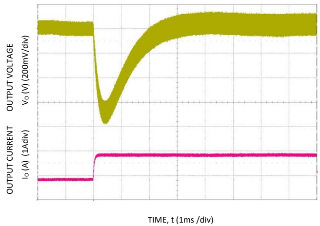
Figure 22. Transient Response to Dynamic Load Change from 0.9A to 1.9A at 12Vin, C_{out}=470uF , C_{Tune}=1000pF , R_{Tune}=30.1k\Omega
