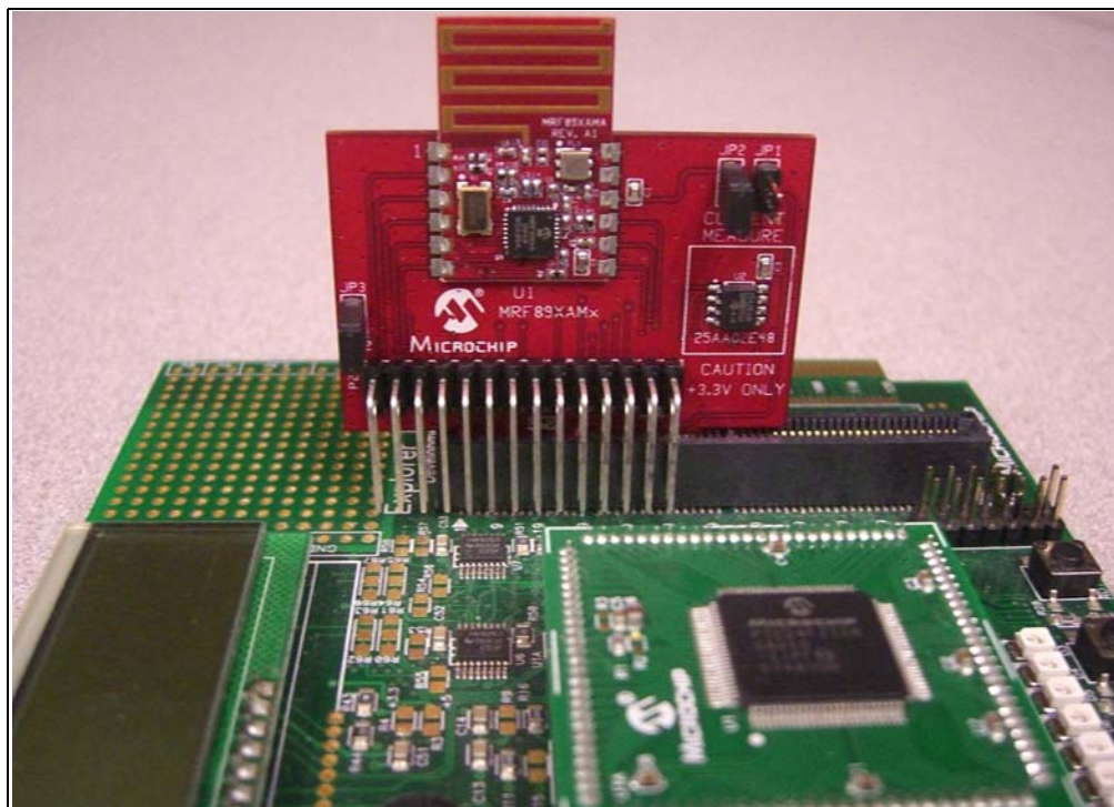
FIGURE 2-2: MRF89XAMxA PICTail™/PICTail PLUS DAUGHTER BOARD PLUGGED INTO EXPLORER 16 DEVELOPMENT BOARD
