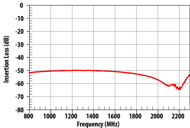
Figure 5. Attenuation, 800 – 2300 MHz
