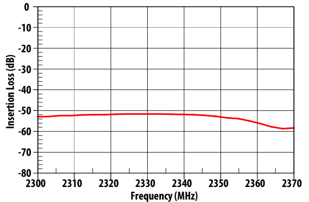
Figure 6. Rejection in LTE Band 40 (2300 – 2370 MHz)
