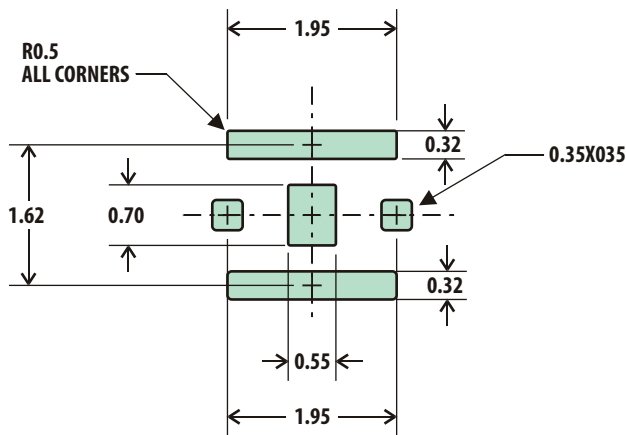
Figure 24. ACFF-1025 Superposed on PCB Layout.
