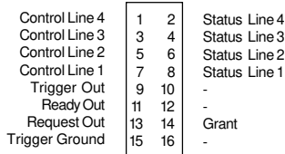
Feature Connector - JP6
