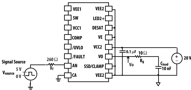
Figure 22. Propagation Delay Test Circuit
