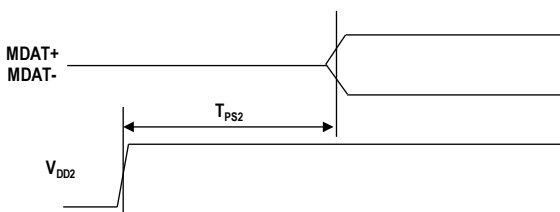
Figure 8. Data delay upon VDD2 startup
