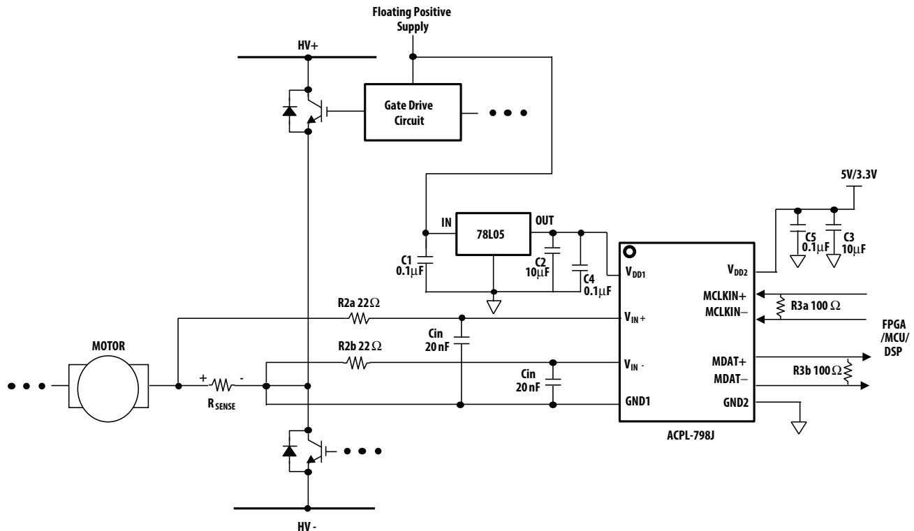
Figure 28. Schematic for three conductor shunt connection.
