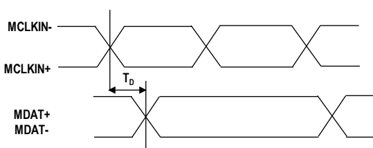
Figure 6. Data propagation delay
