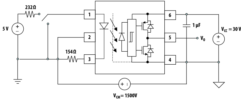
Figure 19 .CMR Test Circuit with Split Resistors Network and Waveforms
