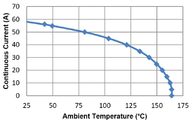
Figure 9: Maximum Continuous Current at a Given T_A
