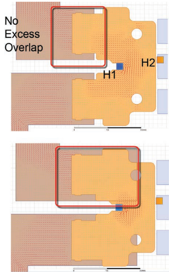
Figure 5: Simulations of ACS780 Leadframe with Different Overlap of the Current Trace and the I_p Bus
